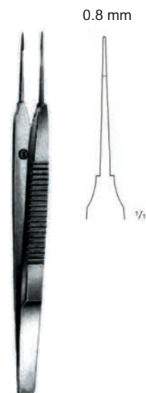
Austin BC-06-173 140 mm
